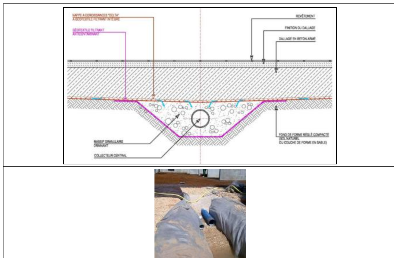
Figure 16 - tranchée drainante
